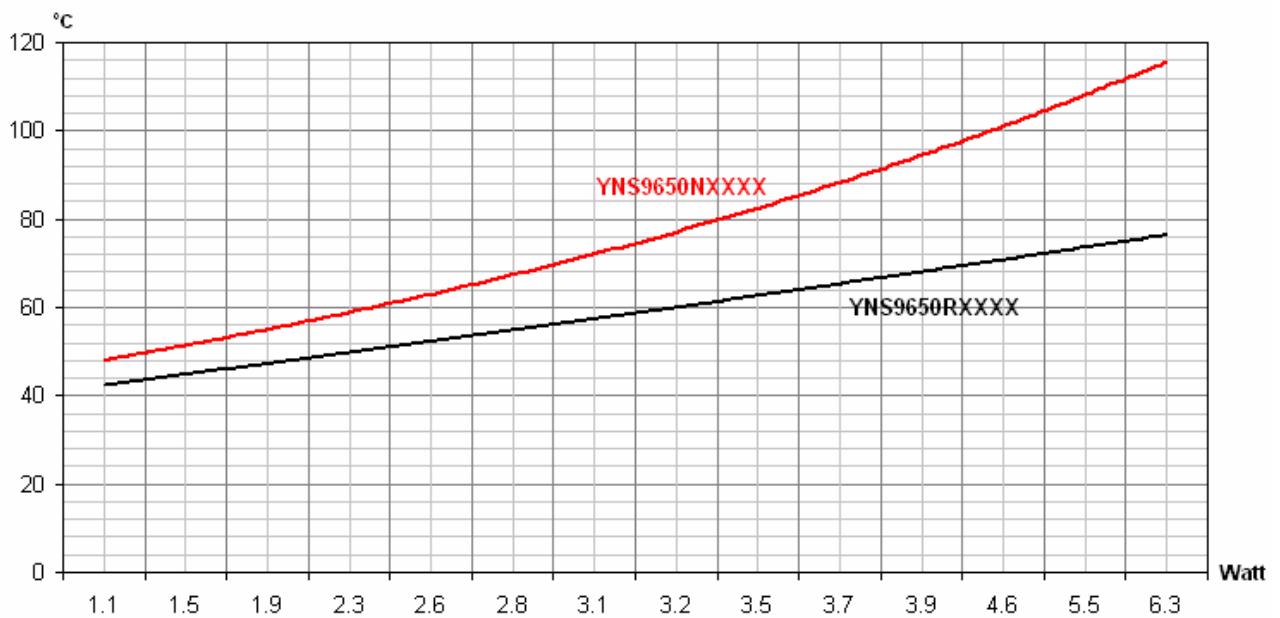
Total Driving Power versus Case Temperature
