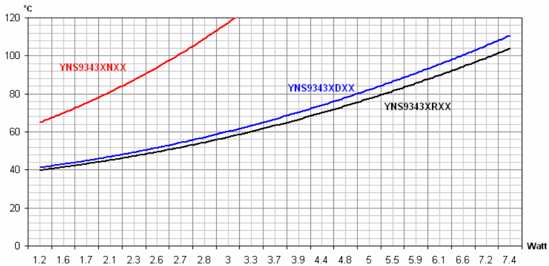
Total Driving Power versus Case Temperature
